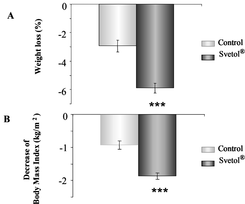
Figure 2: (A) Weight loss (%) and (B) decrease of BMI ( \text{kg}/\text{m}^2 ) after 60 days treatment. Values are means \pm SEM, n = 20 for control group, n = 30 for Svetol® group. Means are significantly different (*, p < 0.001 vs. control group).
